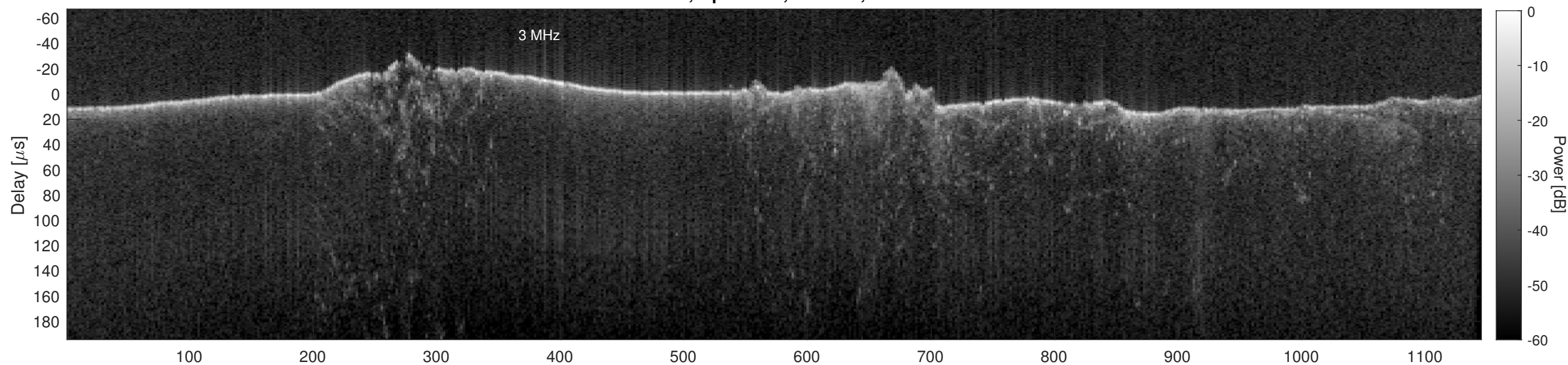
Orbit 17453, Cluttergram
