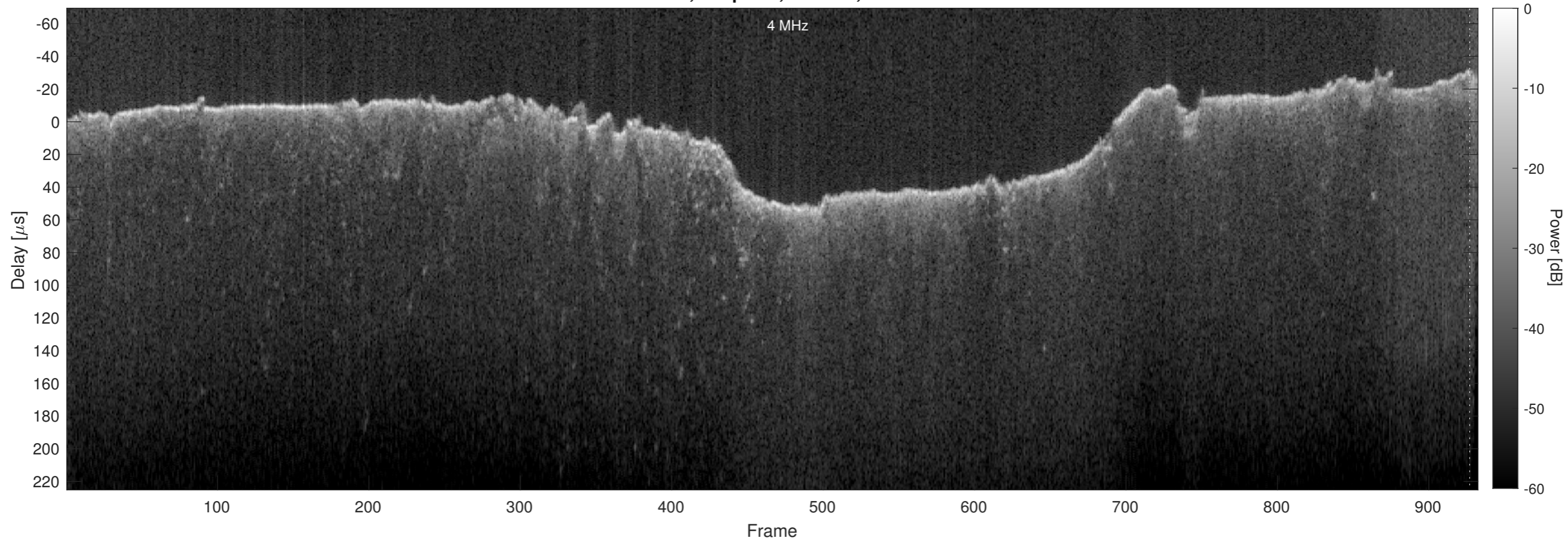
Orbit 17455, Chapman, Window, Channel 2
