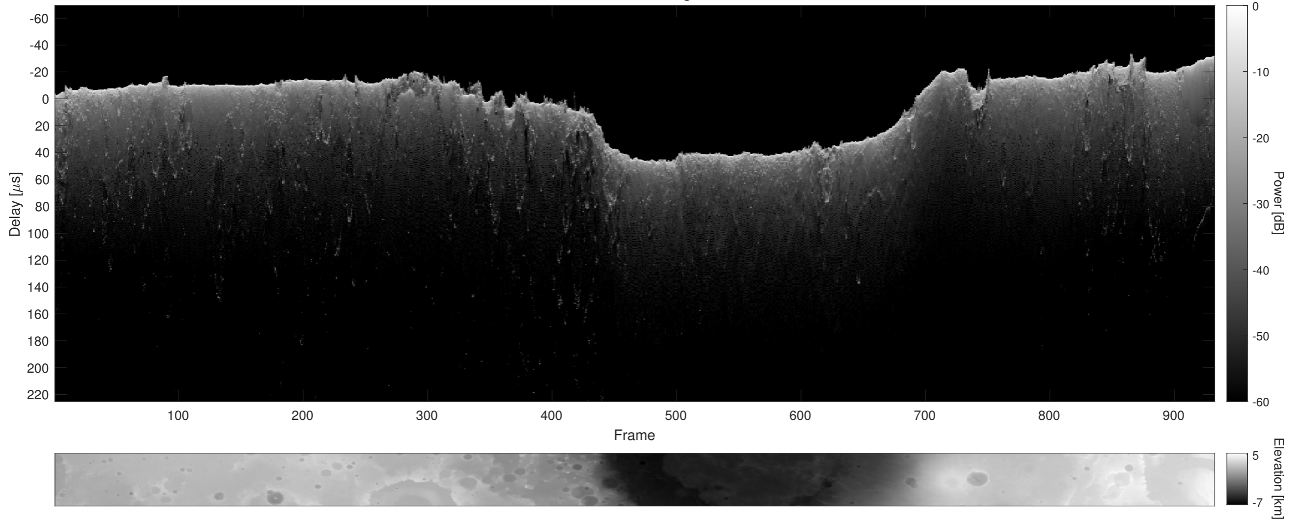
Orbit 17455, Cluttergram
