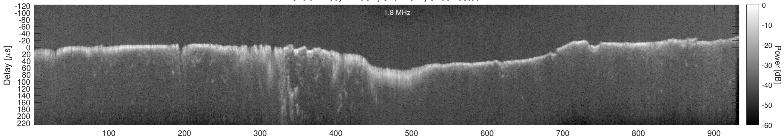
Orbit 17455, Window, Channel 2, Chapman
