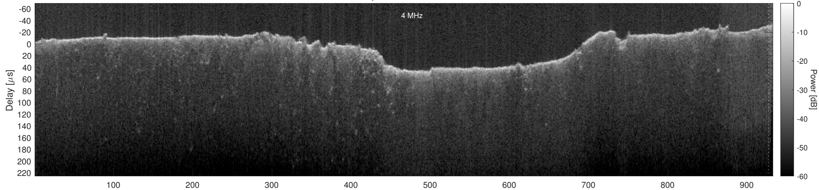
Orbit 17455, Optimized, Window, Channel 2
