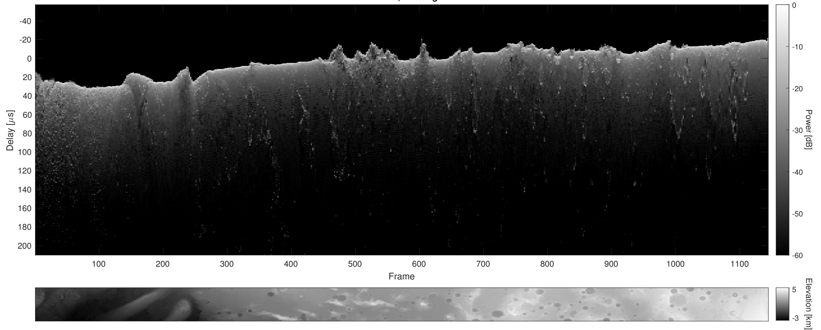
Orbit 17457, Cluttergram
