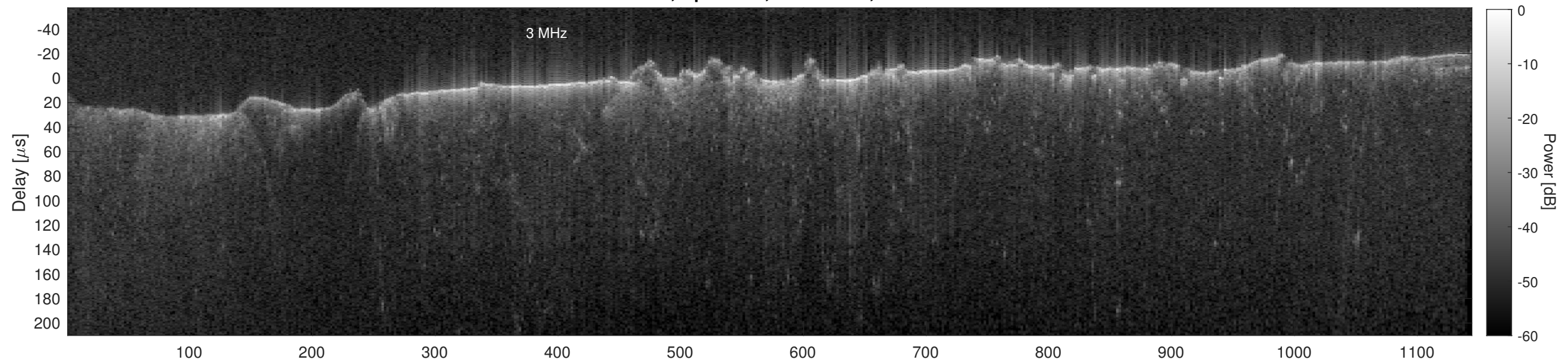
Orbit 17457, Cluttergram
