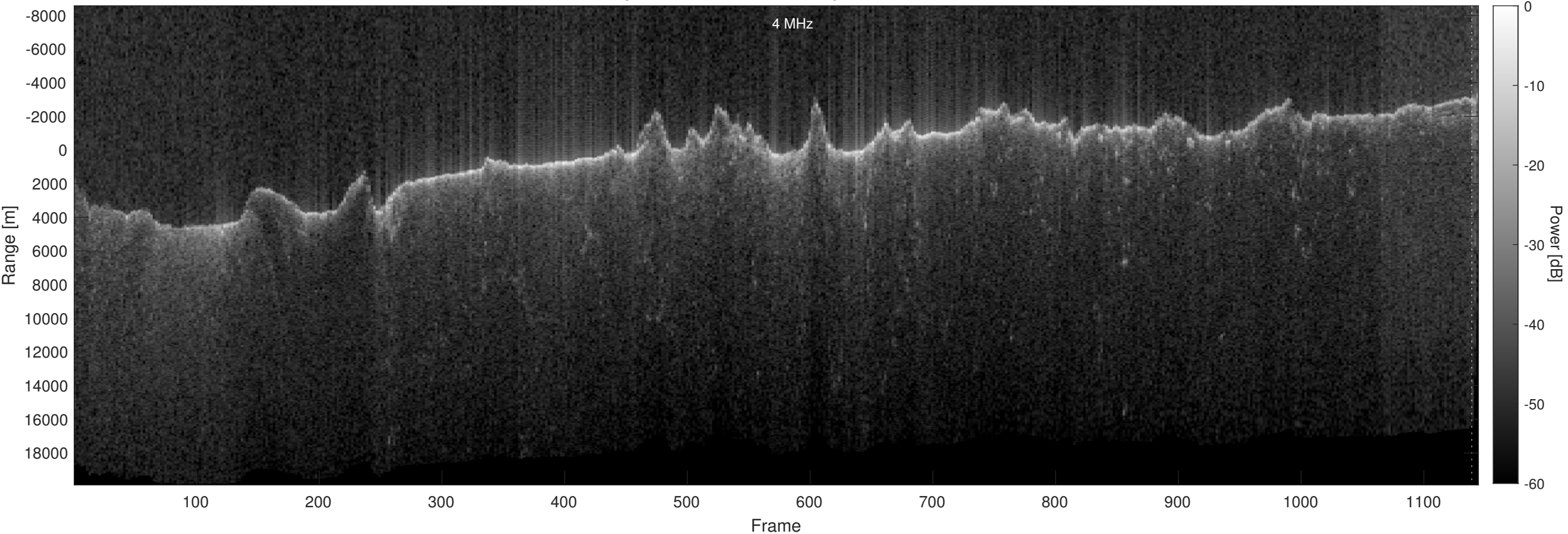
Orbit 17457, Optimized, No Window, Depth-Corrected, Channel 2
