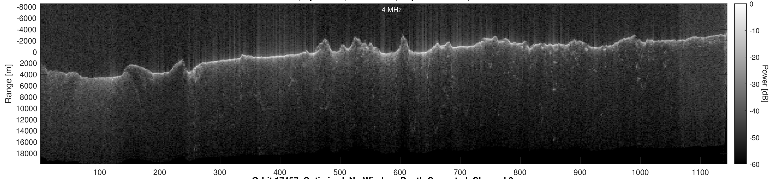
Orbit 17457, Optimized, No Window, Depth-Corrected, Channel 2
