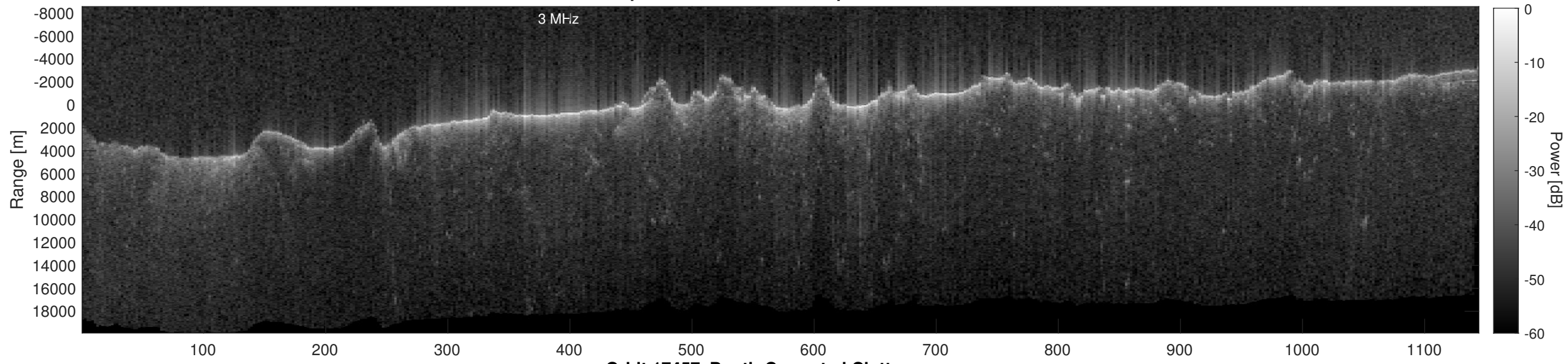
Orbit 17457, Depth-Corrected Cluttergram
