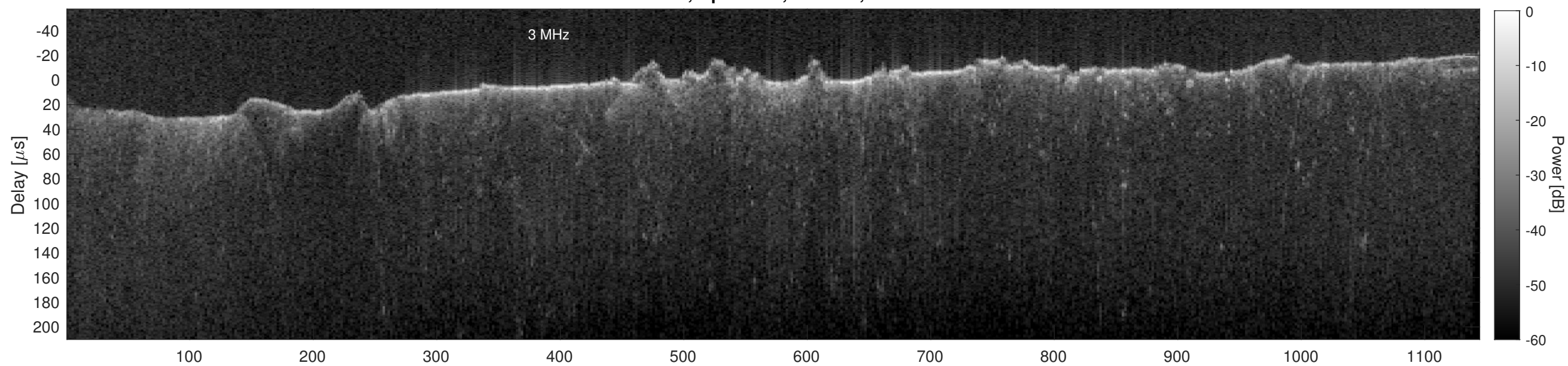
Orbit 17457, Cluttergram
