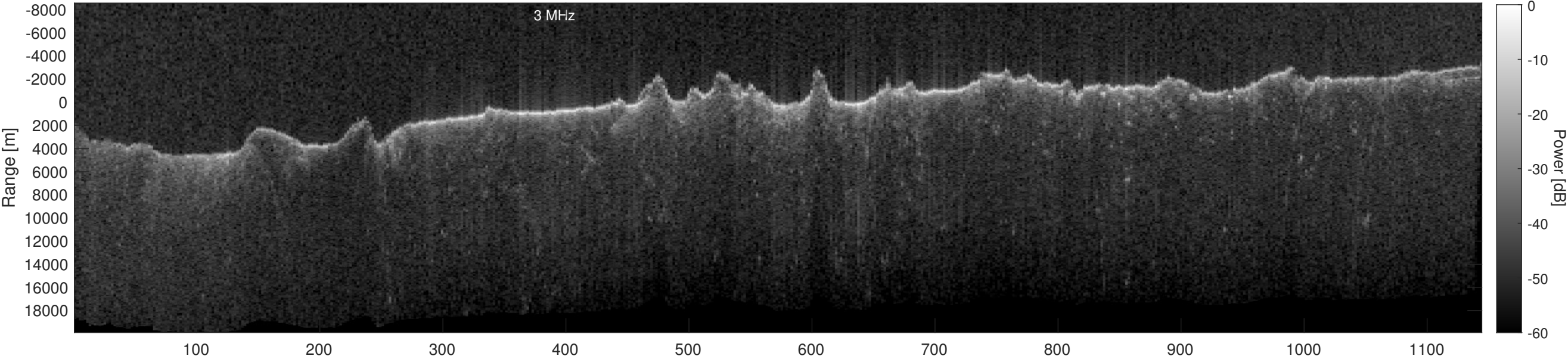
Orbit 17457, Depth-Corrected Cluttergram
