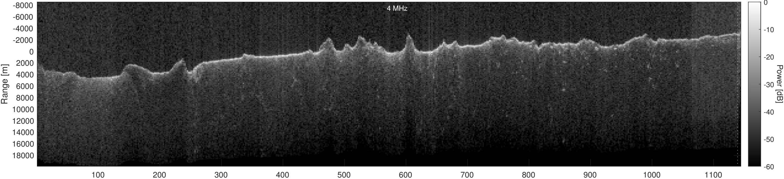
Orbit 17457, Optimized, Window, Depth-Corrected, Channel 2
