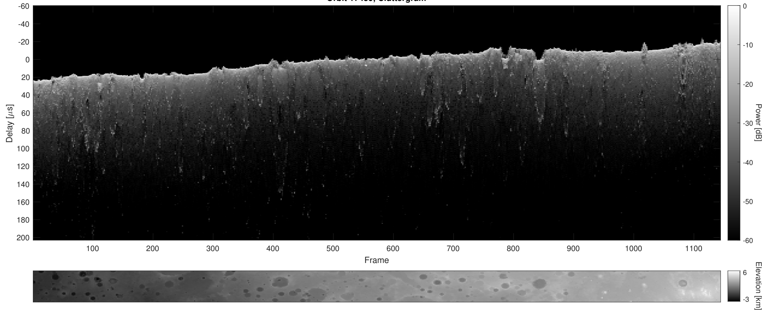
Orbit 17459, Cluttergram
