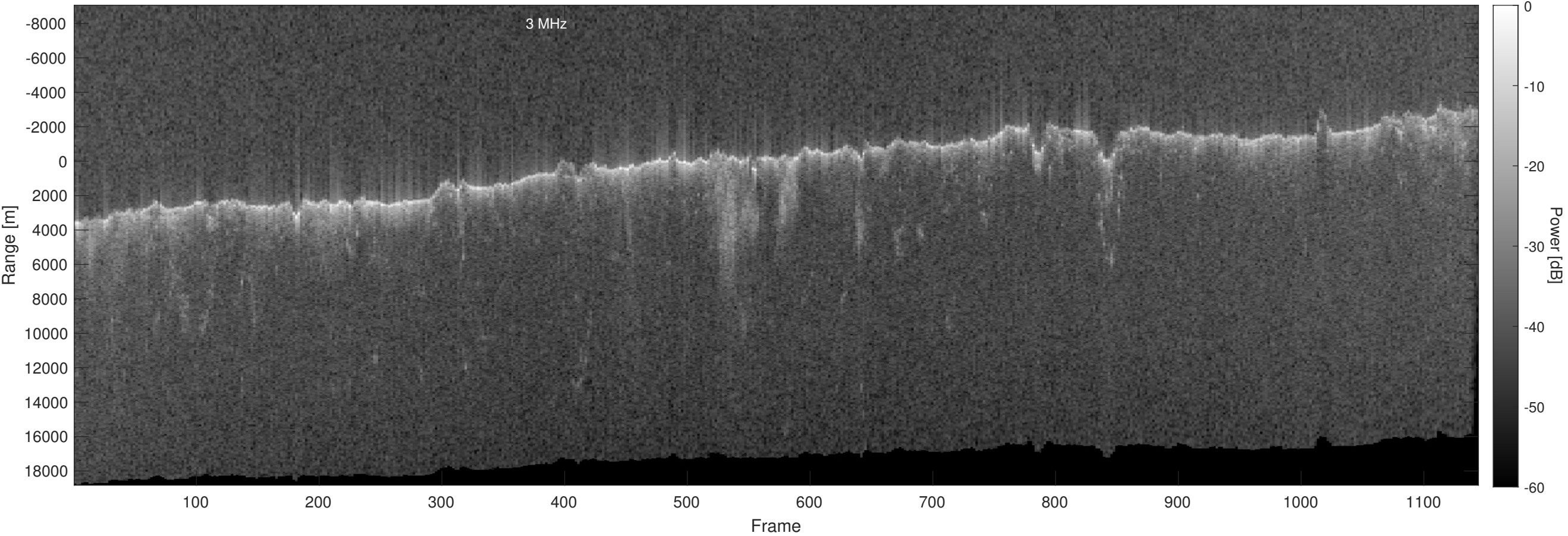
Orbit 17459, Optimized, No Window, Depth-Corrected, Channel 2
