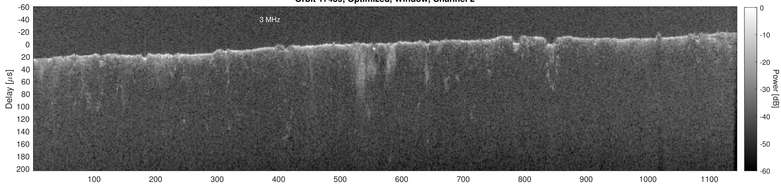
Orbit 17459, Cluttergram
