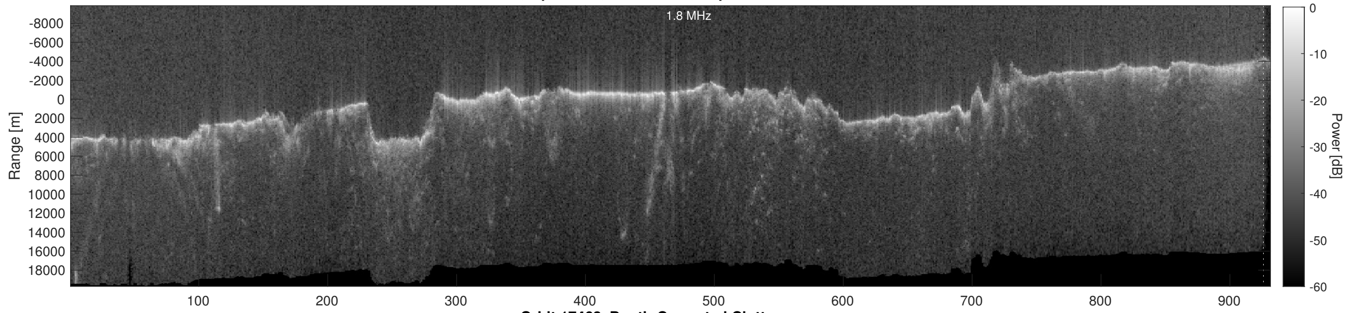
Orbit 17463, Depth-Corrected Cluttergram
