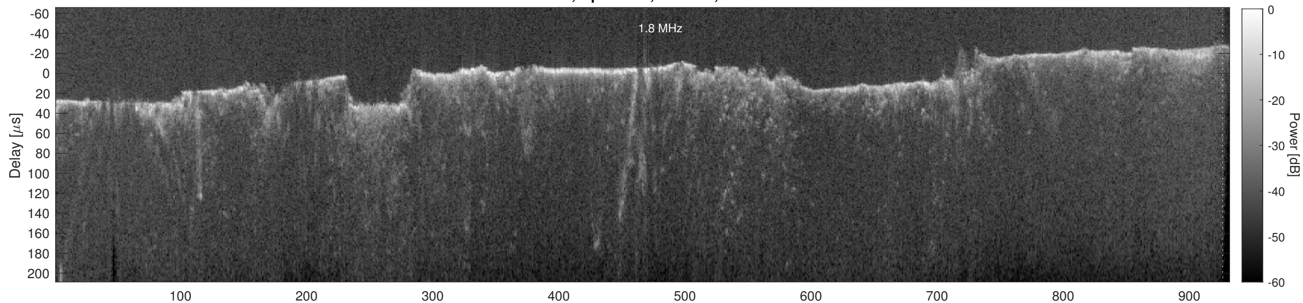
Orbit 17463, Cluttergram
