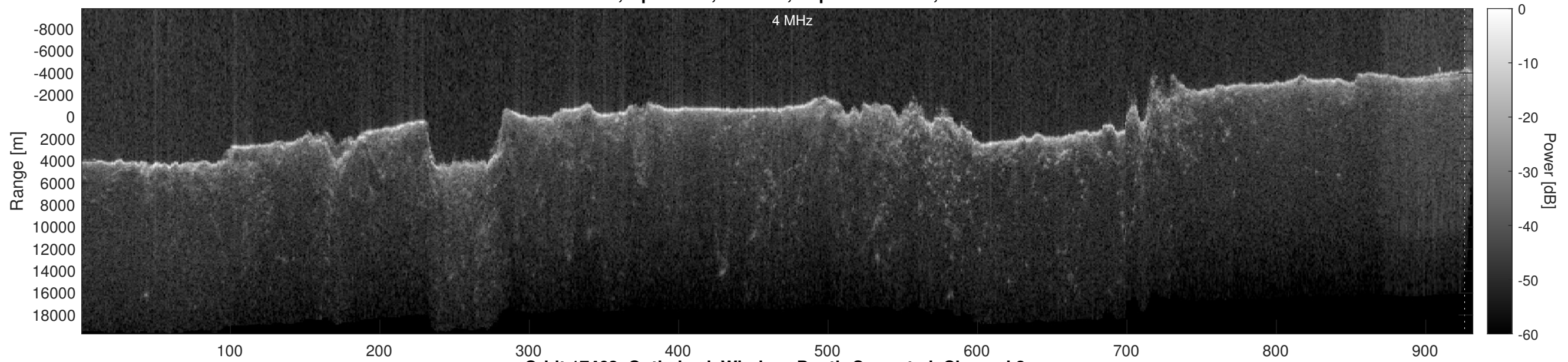
Orbit 17463, Optimized, Window, Depth-Corrected, Channel 2
