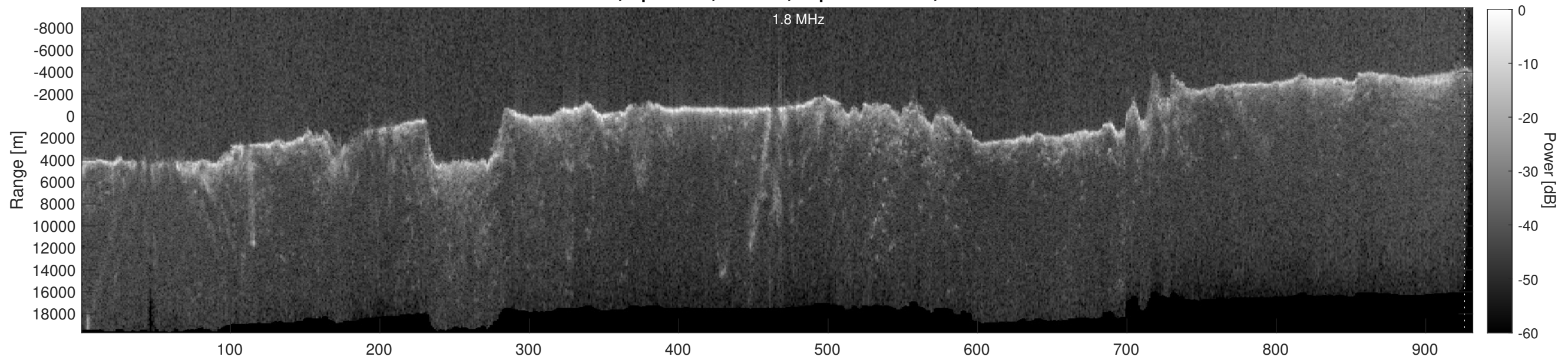
Orbit 17463, Depth-Corrected Cluttergram
