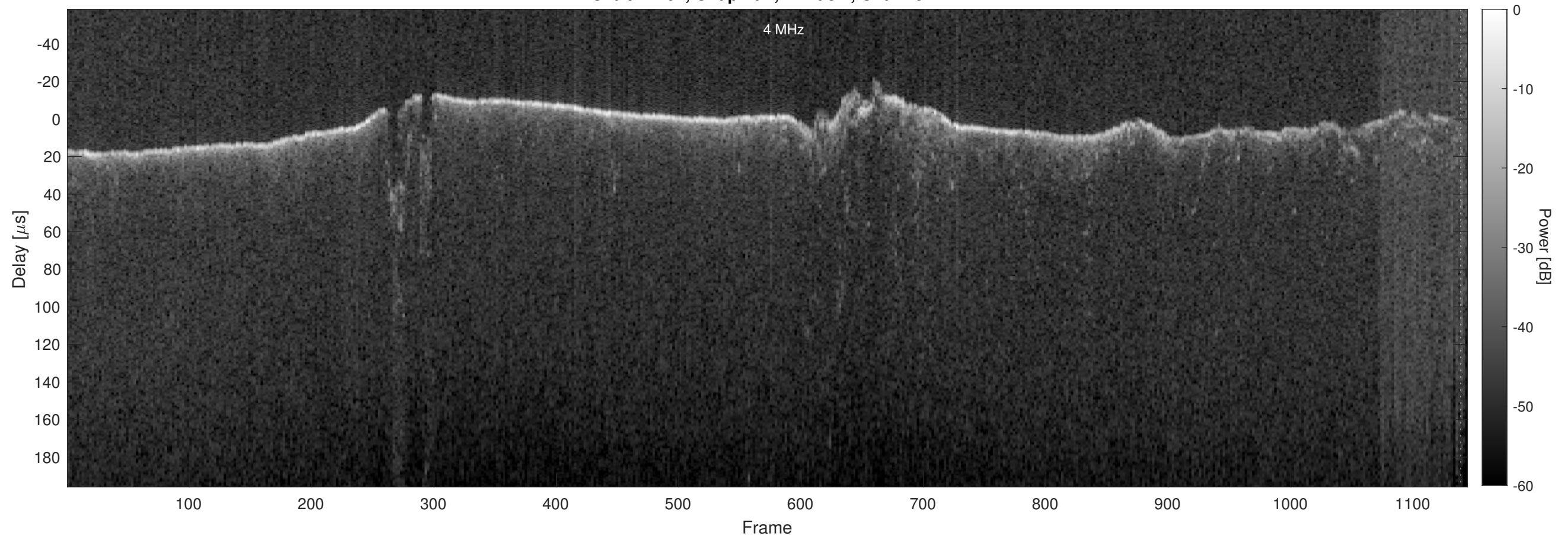
Orbit 17467, Chapman, Window, Channel 2
