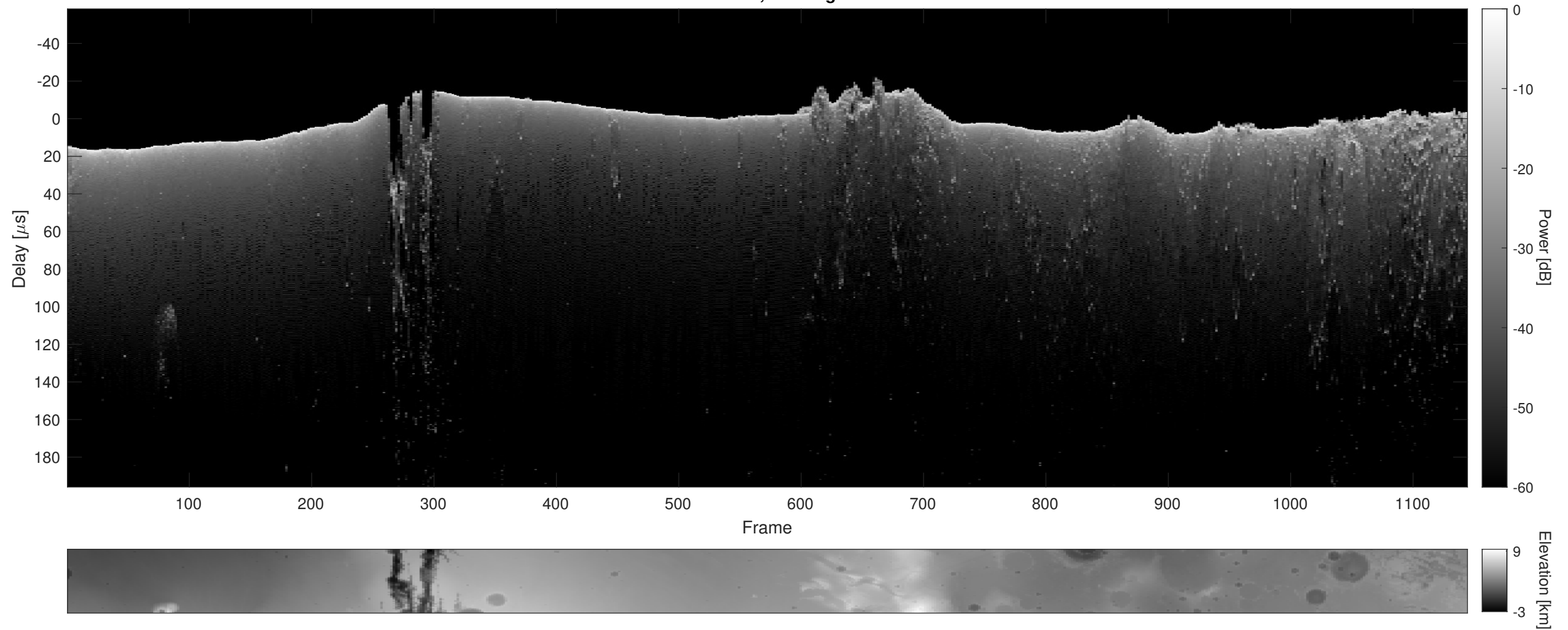
Orbit 17467, Cluttergram
