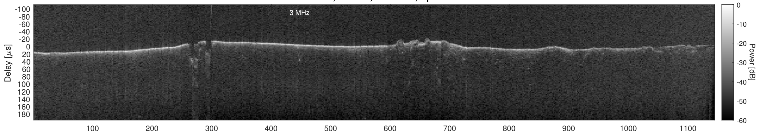
Orbit 17467, Cluttergram
