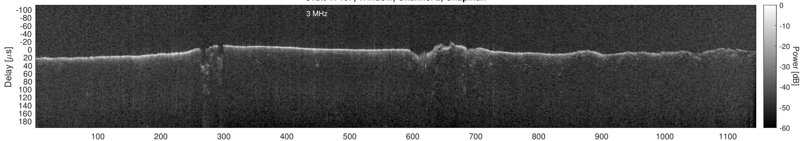
Orbit 17467, Window, Channel 2, Optimized
