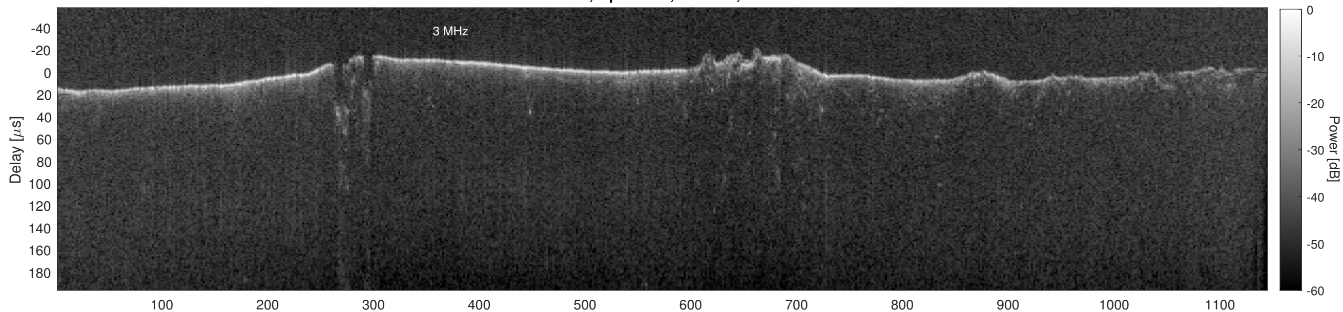
Orbit 17467, Cluttergram
