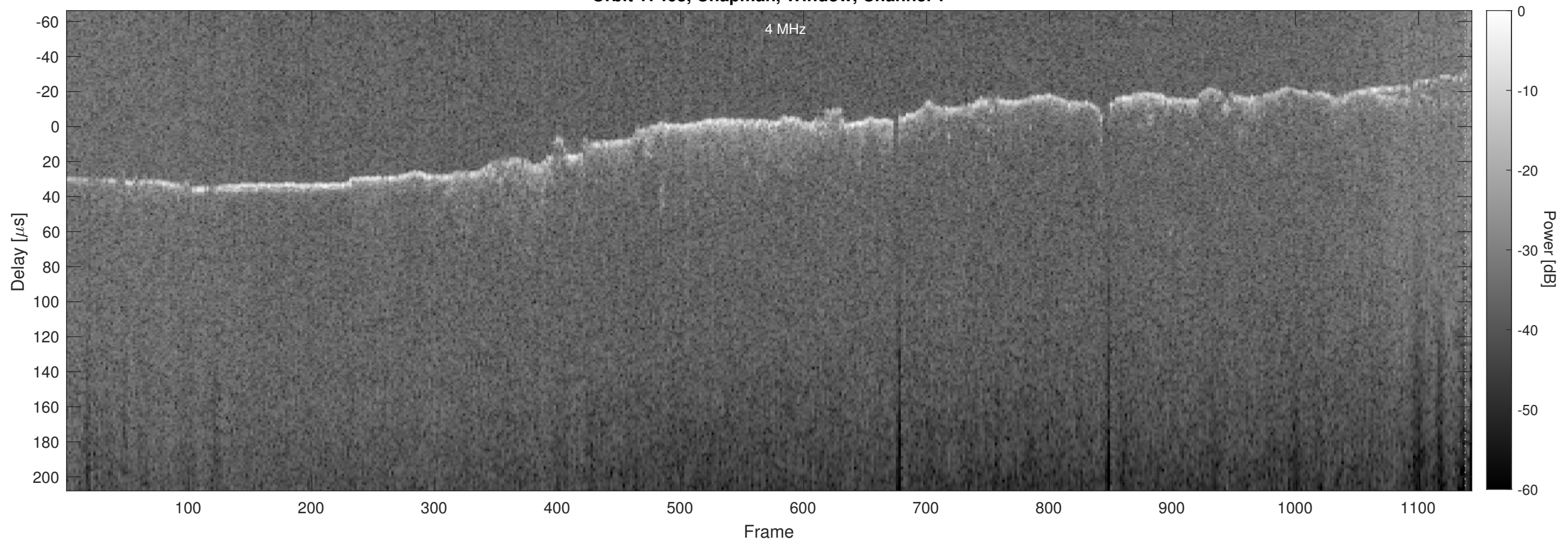
Orbit 17468, Chapman, Window, Channel 2
