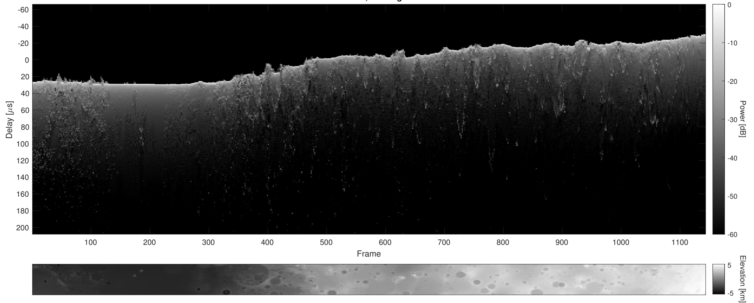
Orbit 17468, Cluttergram
