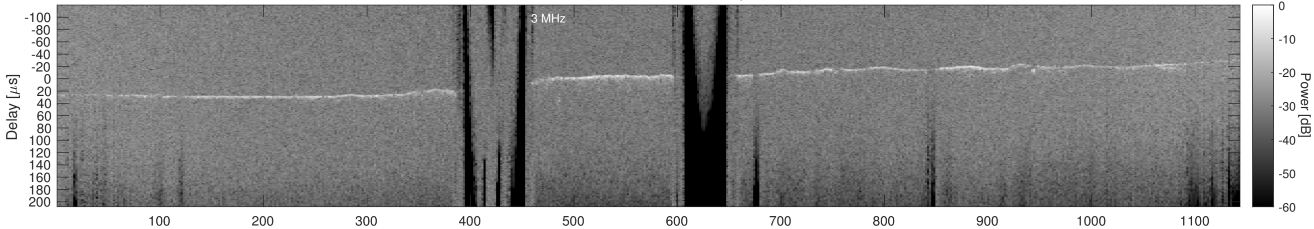
Orbit 17468, Cluttergram
