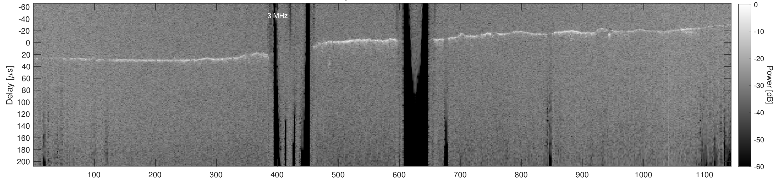
Orbit 17468, Cluttergram
