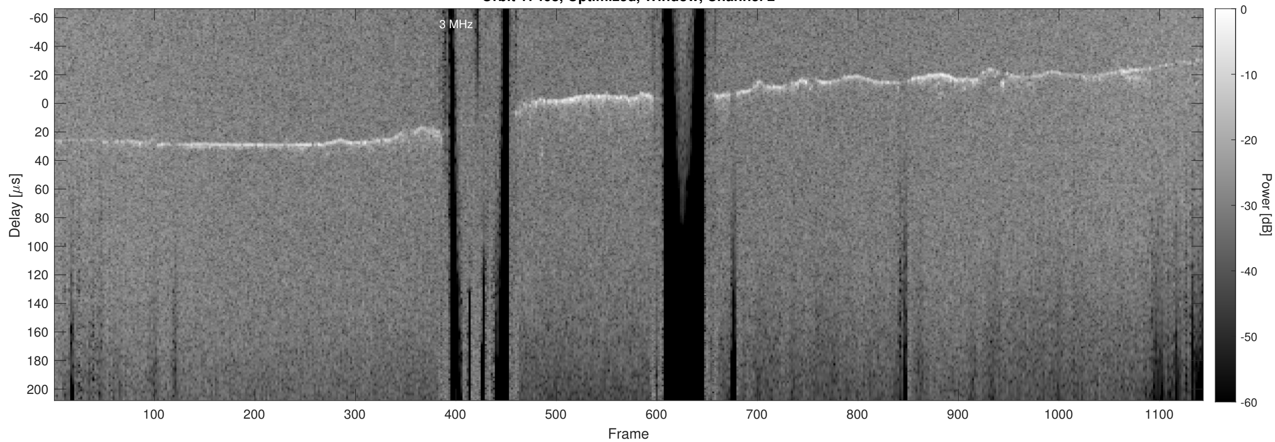
Orbit 17468, Optimized, Window, Channel 2
