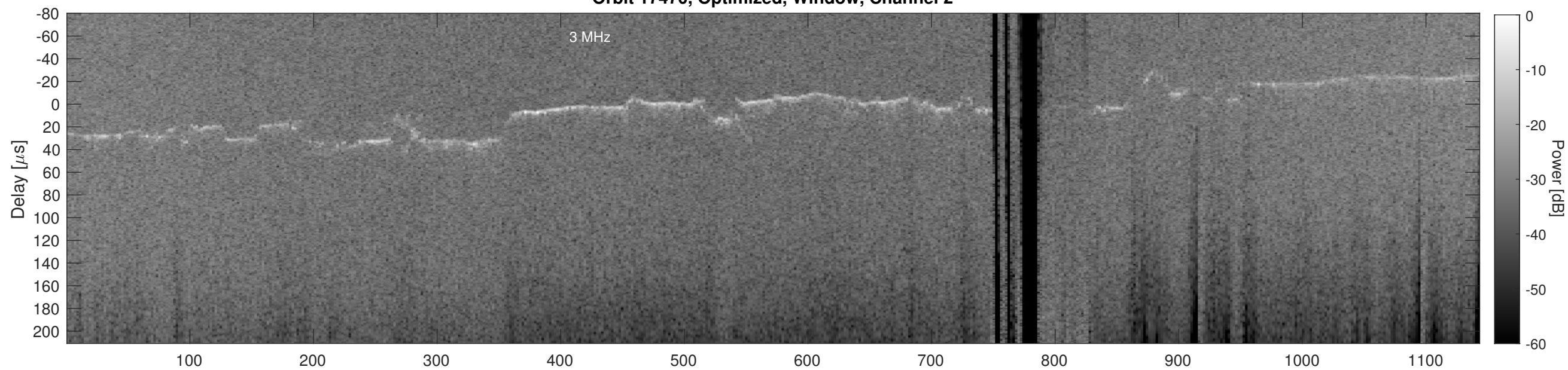
Orbit 17470, Cluttergram
