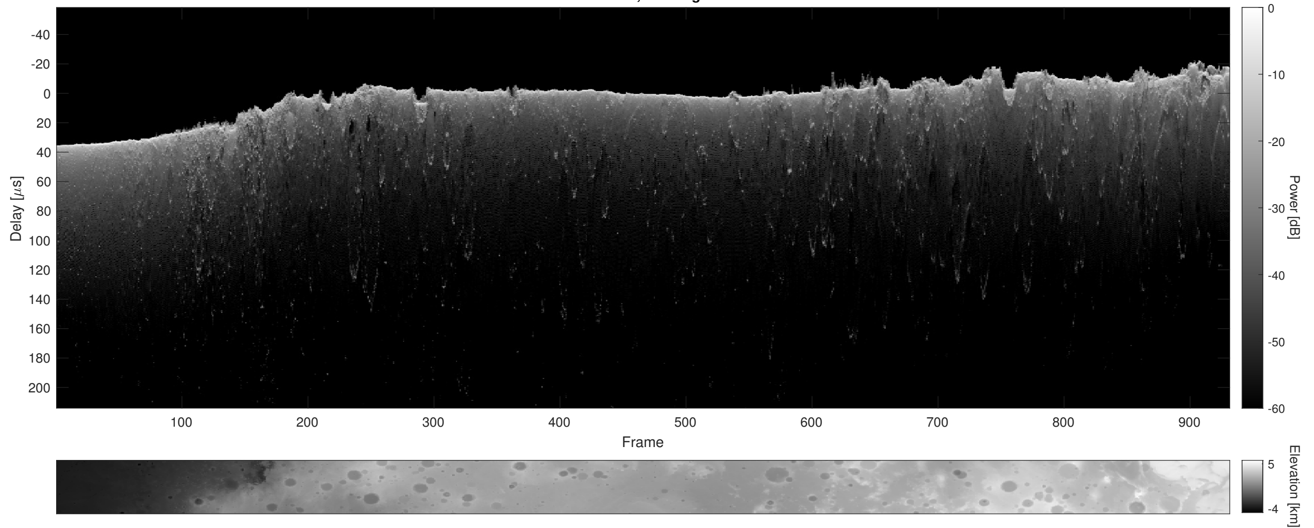
Orbit 17472, Cluttergram
