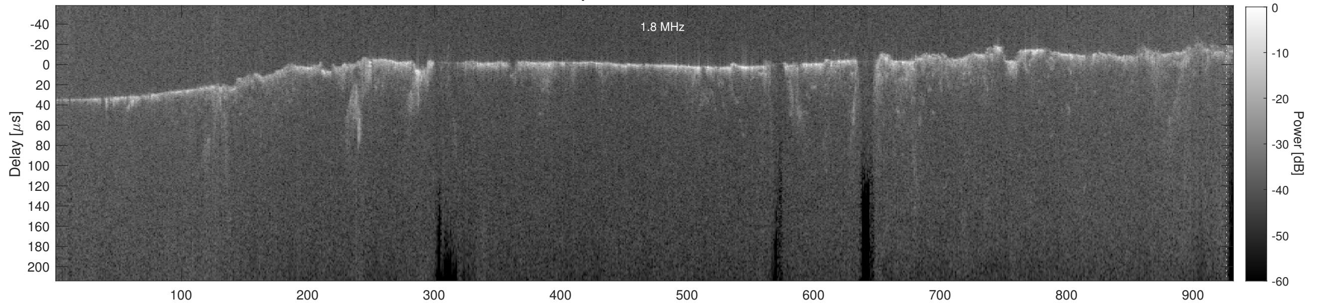
Orbit 17472, Cluttergram
