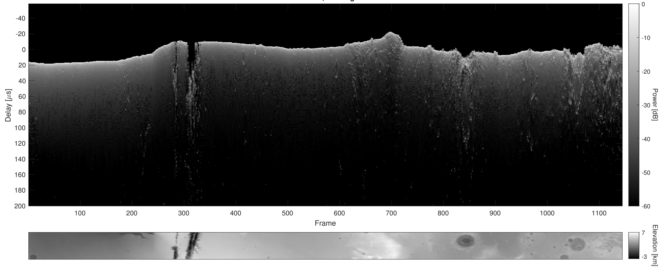
Orbit 17474, Cluttergram
