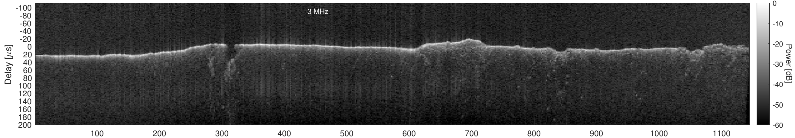
Orbit 17474, Window, Channel 2, Optimized
