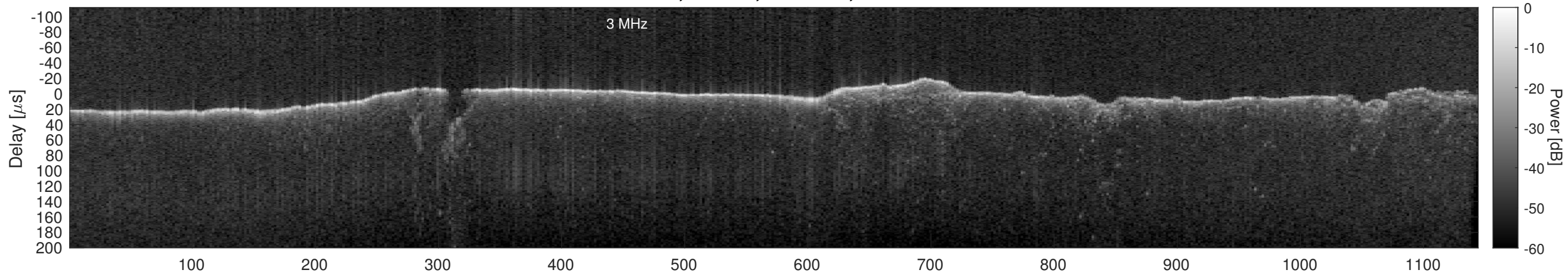
Orbit 17474, Window, Channel 2, Chapman
