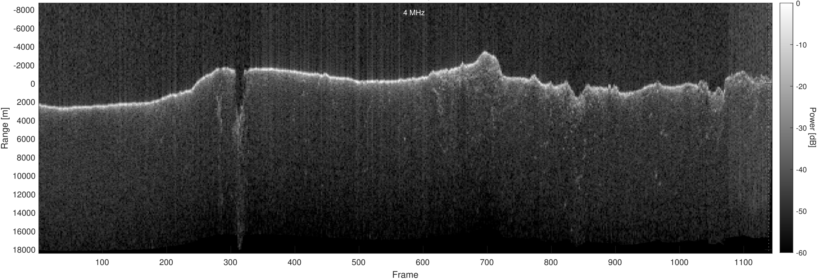
Orbit 17474, Optimized, Window, Depth-Corrected, Channel 2
