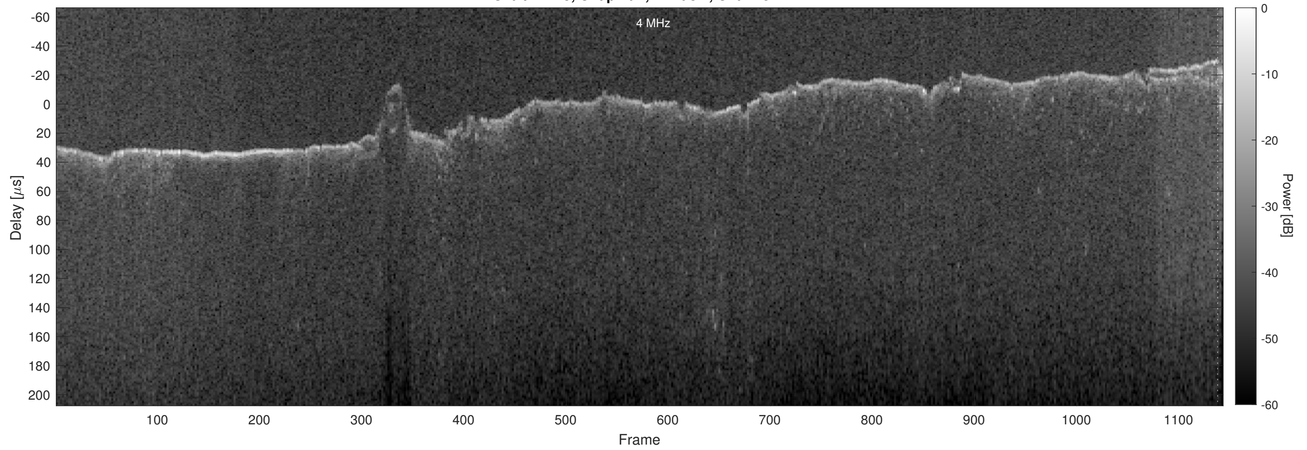
Orbit 17475, Chapman, Window, Channel 2
