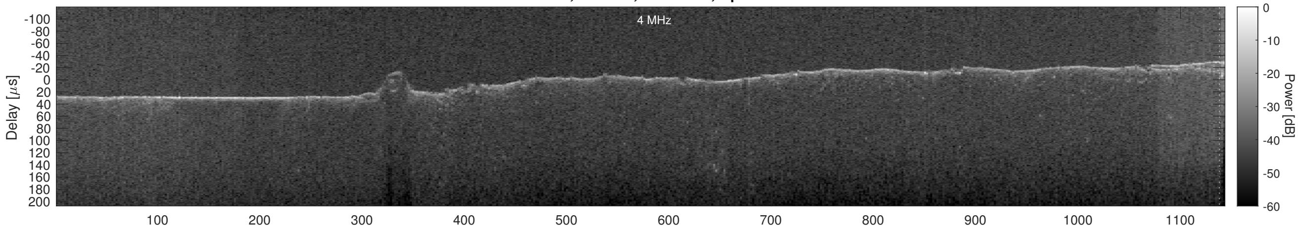
Orbit 17475, Cluttergram
