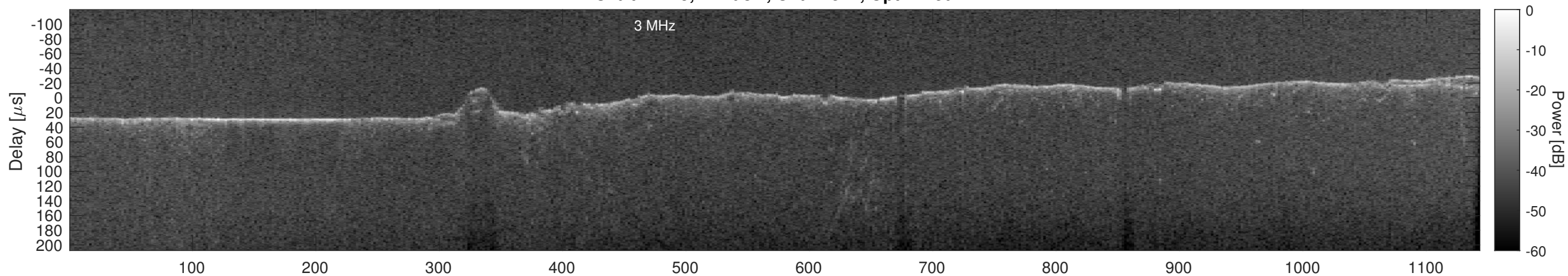
Orbit 17475, Cluttergram
