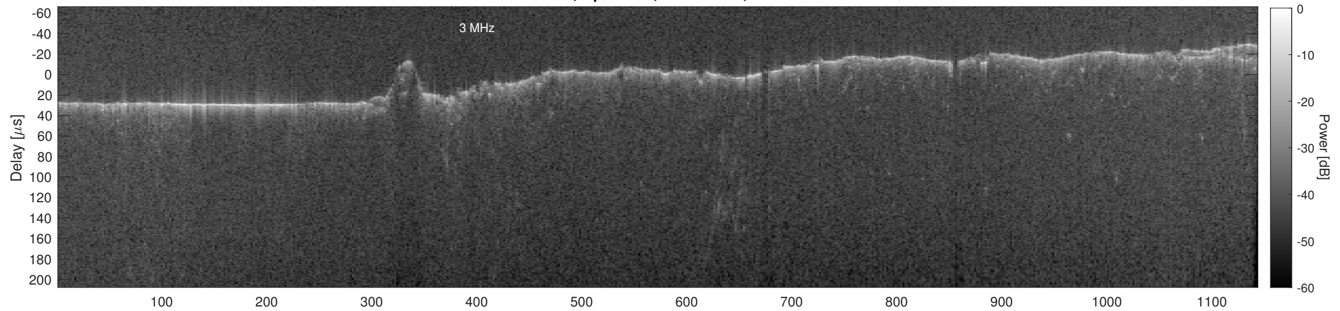
Orbit 17475, Cluttergram
