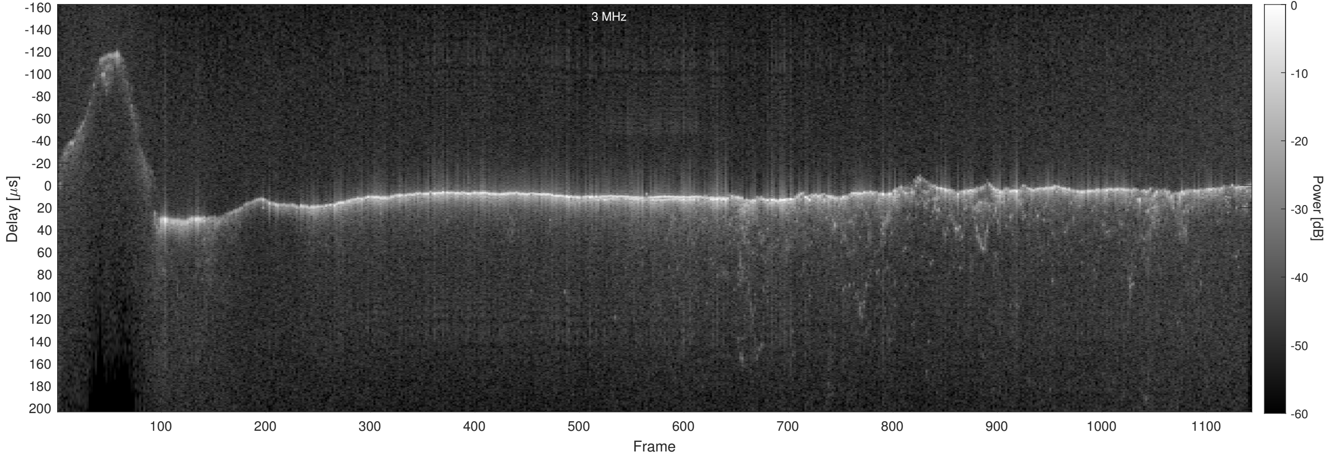
Orbit 17478, Chapman, No Window, Channel 2
