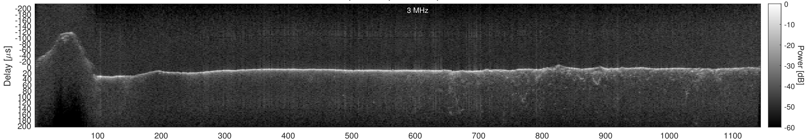
Orbit 17478, Window, Channel 2, Chapman
