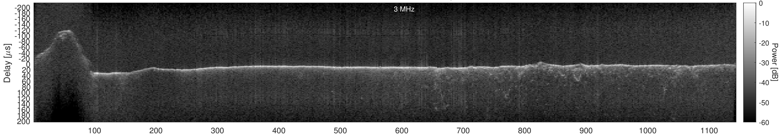
Orbit 17478, Window, Channel 2, Optimized
