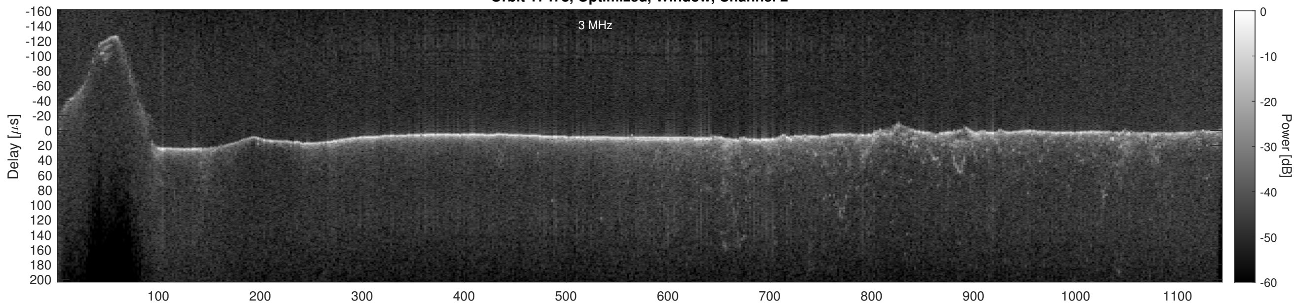
Orbit 17478, Cluttergram
