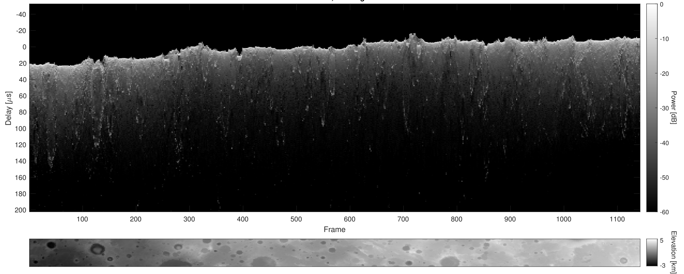
Orbit 17480, Cluttergram
