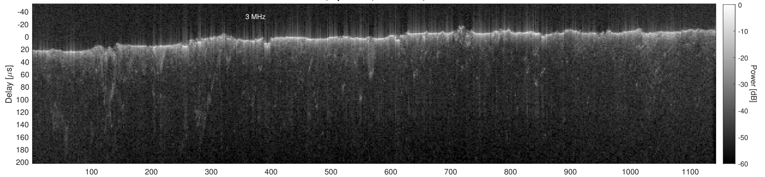
Orbit 17480, Cluttergram
