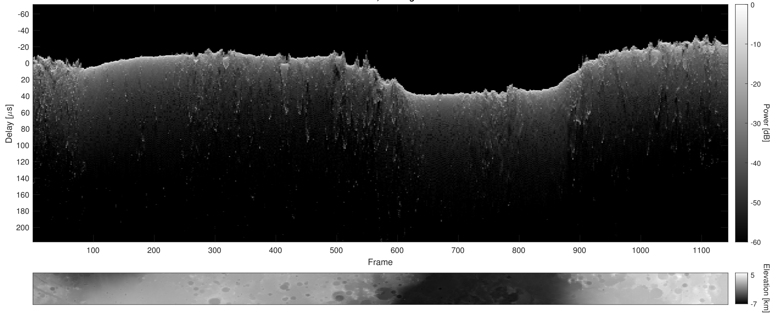
Orbit 17483, Cluttergram
