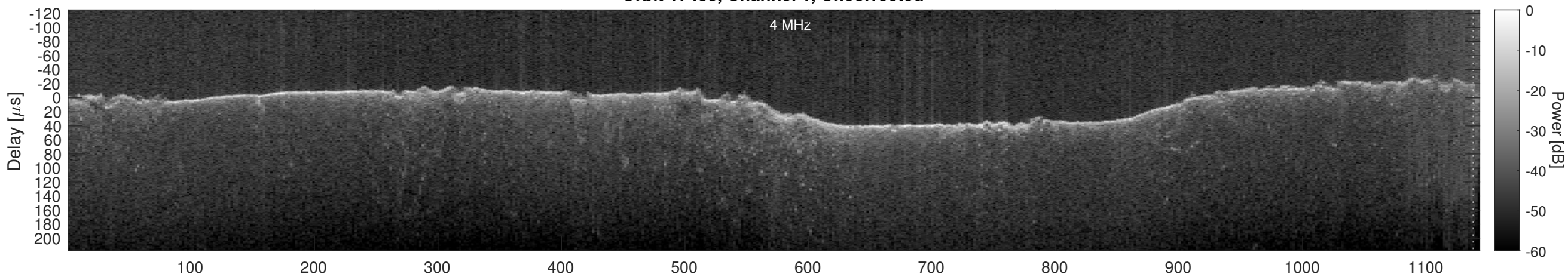
Orbit 17483, Window, Channel 1, Chapman
