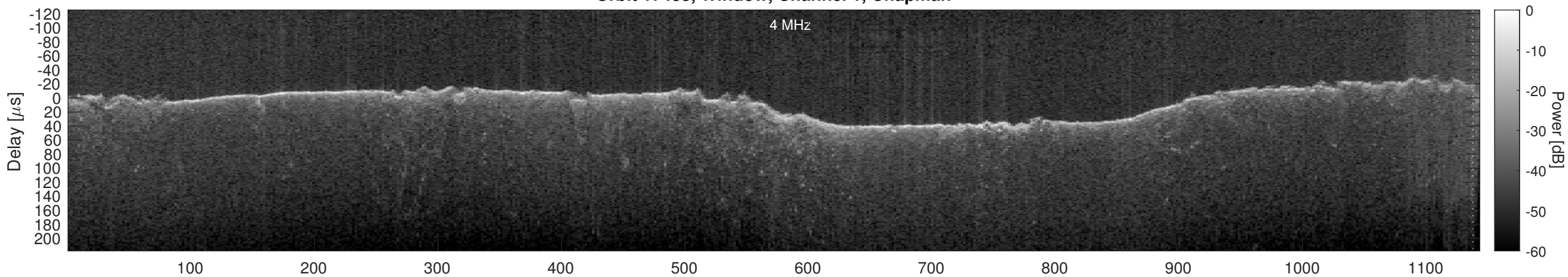
Orbit 17483, Window, Channel 1, Optimized
