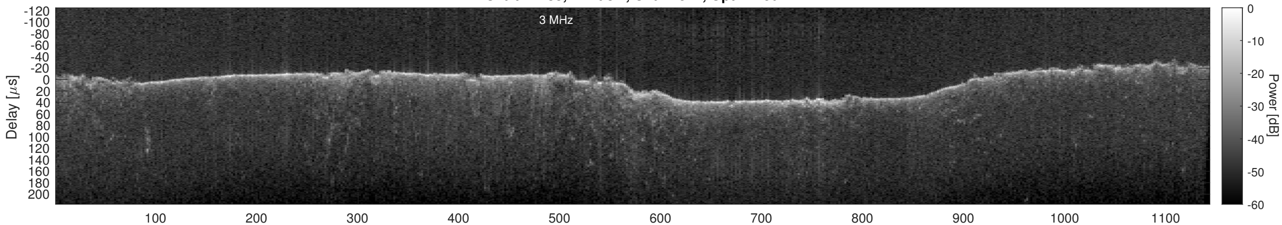
Orbit 17483, Cluttergram
