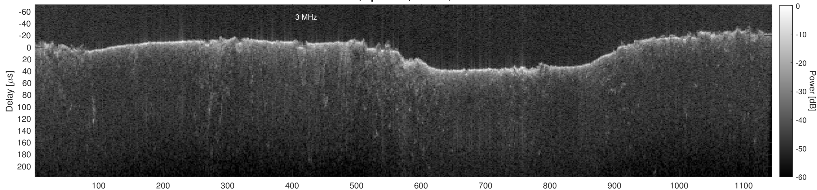
Orbit 17483, Cluttergram
