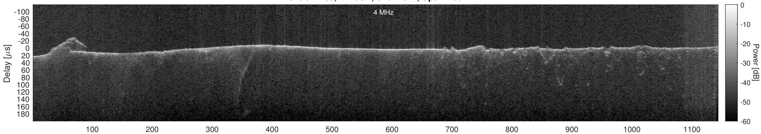
Orbit 17485, Cluttergram
