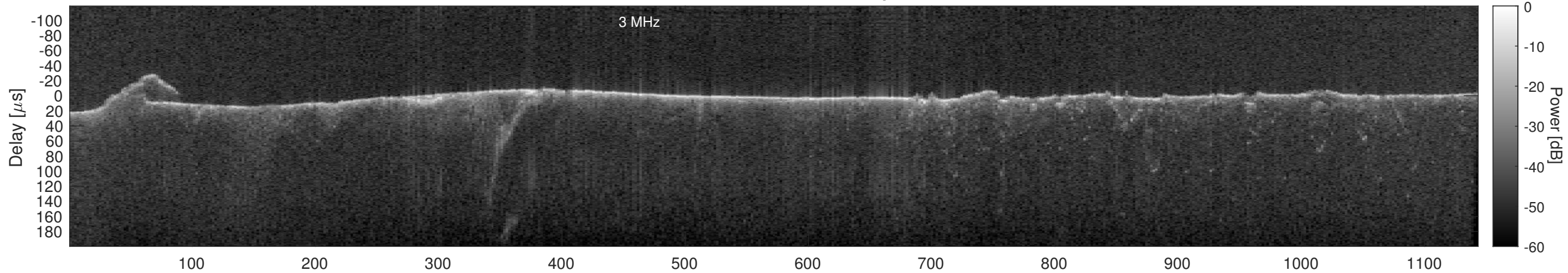
Orbit 17485, Cluttergram
