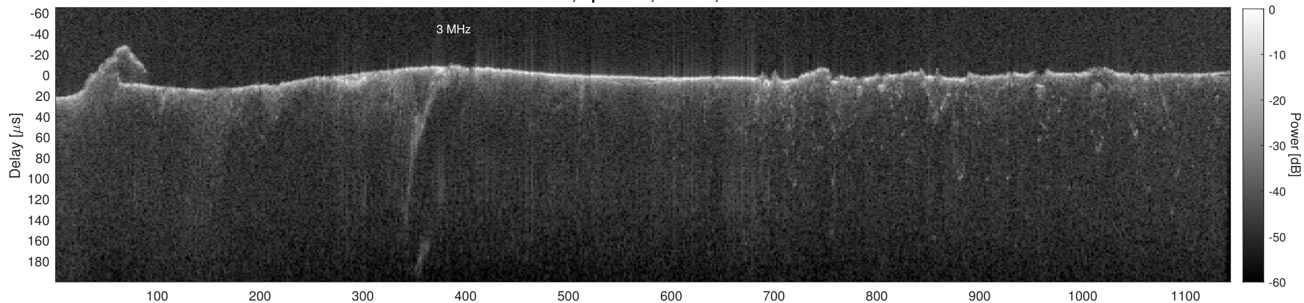
Orbit 17485, Cluttergram
