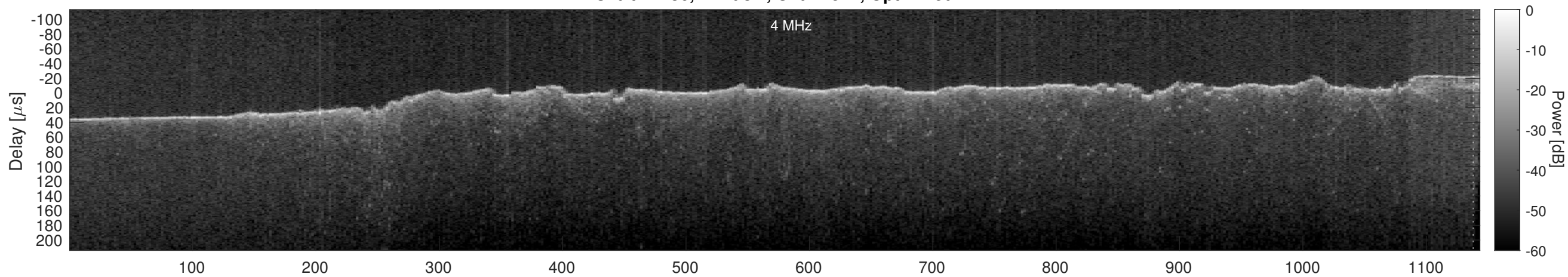
Orbit 17486, Cluttergram
