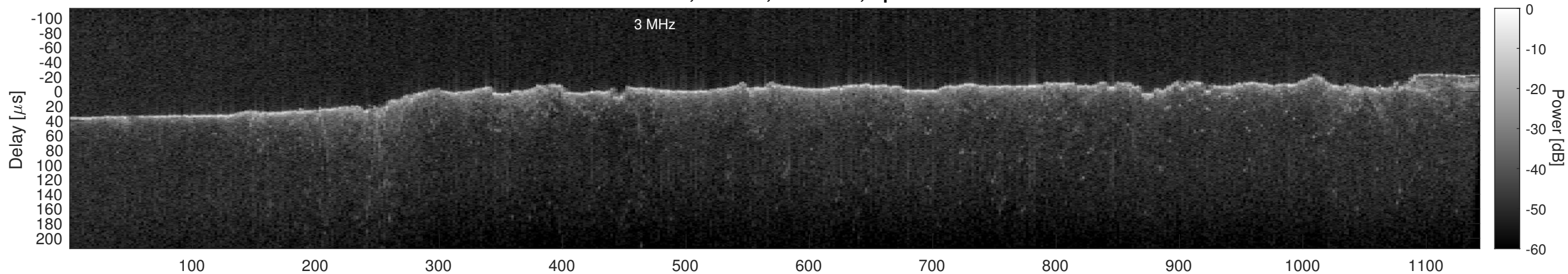
Orbit 17486, Cluttergram
